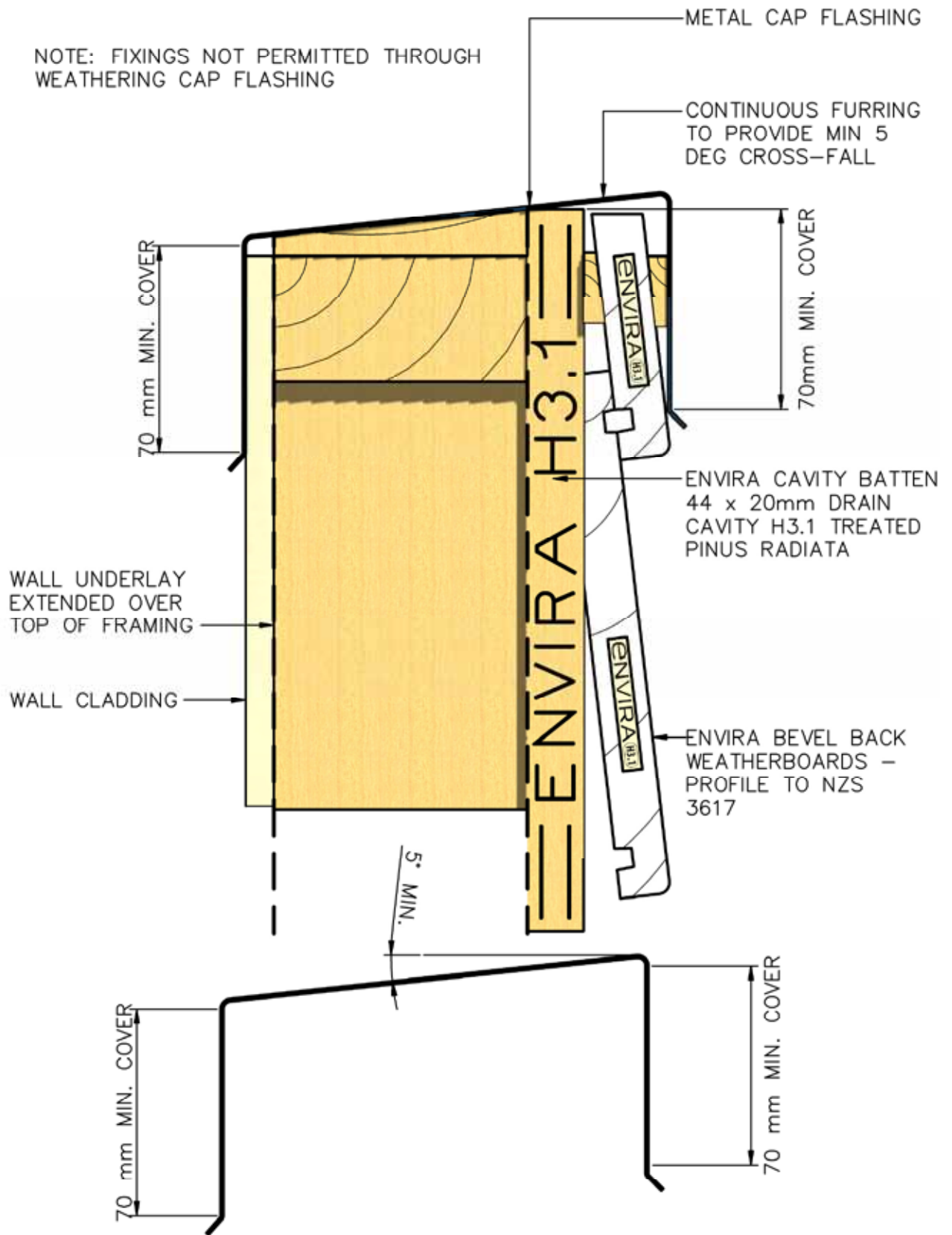
FLASHING DIMENSIONS
